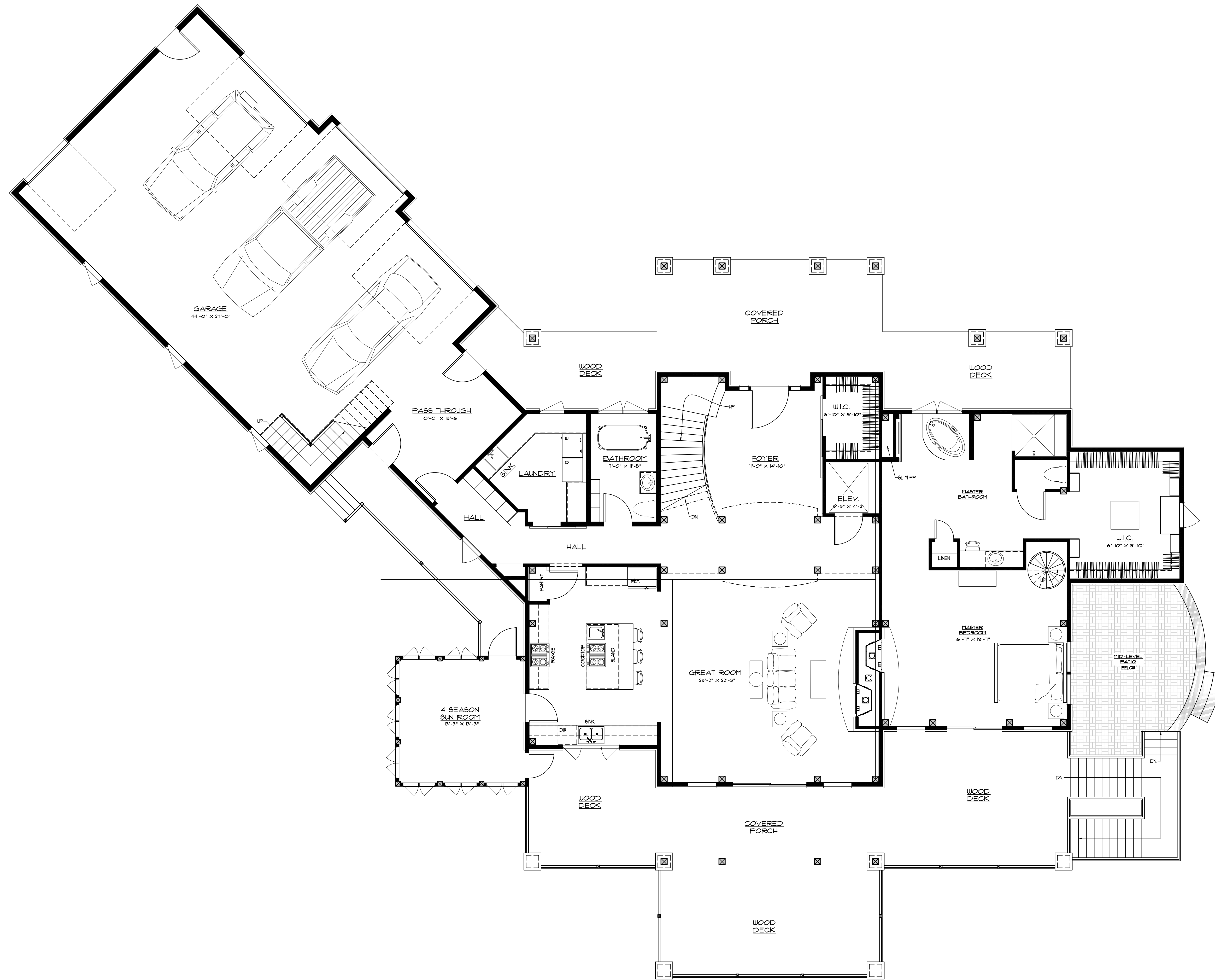
PLAN VIEW (1ST FLOOR) 3/16" = 1'-0"
